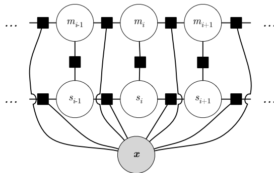
Figure 1: Double-chainned CRF expressed as a factor graph: \mathbf{x} is the whole sentence. For a token in position i , its MWE label is m_i and its supersense tag is s_i .
