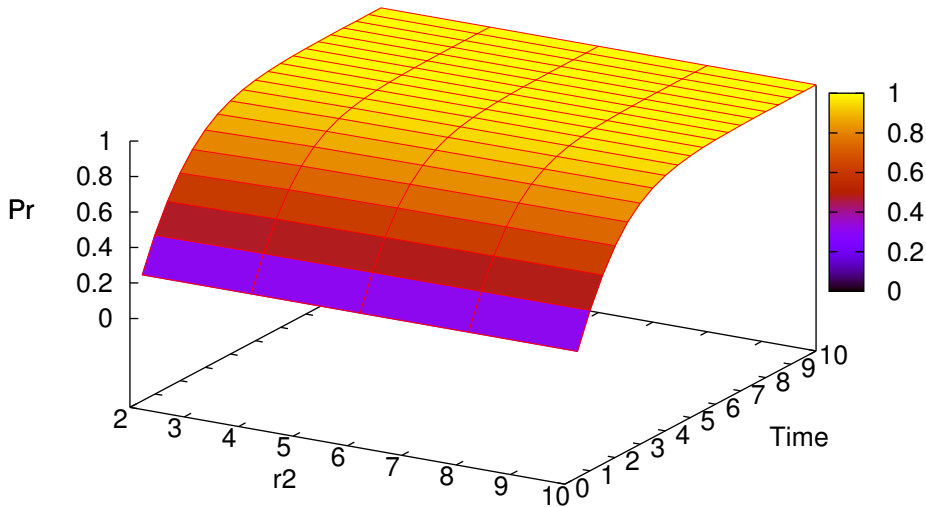
Sensitivity of cumulative distribution function to r^2
