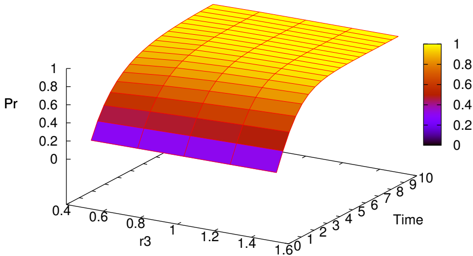
Sensitivity of cumulative distribution function to r3
