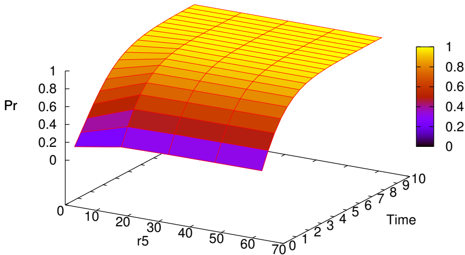
Sensitivity of cumulative distribution function to r5
