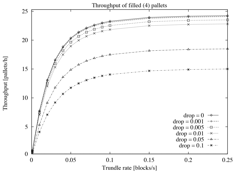
Figure 1: Throughput (full pallets/hour) of the workcell dependent on trundle rate
