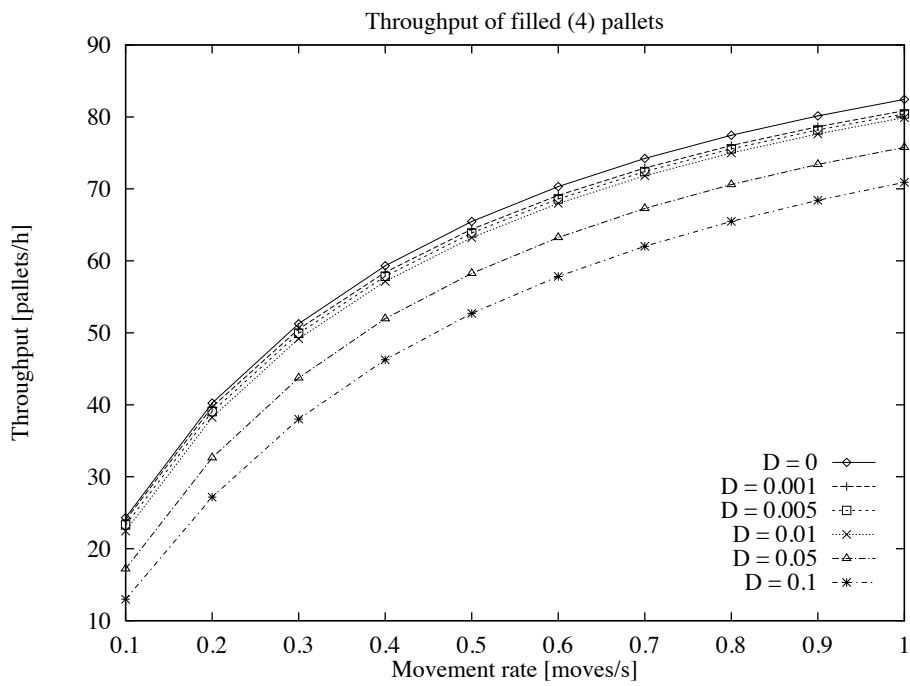
Figure 2: Throughput (full pallets/hour) of the workcell dependent on movement rate
